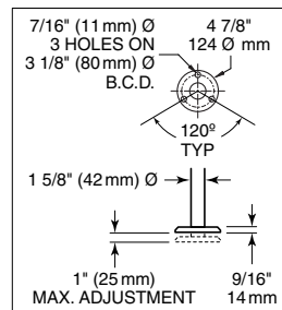
FLANGED FOOT DETAIL
